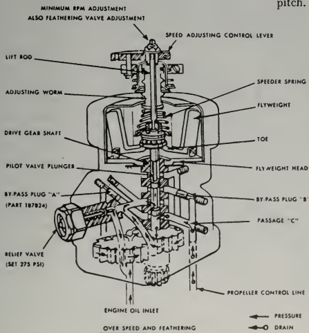
FIGURE 7-16. Woodward Governor X210,000 Series
